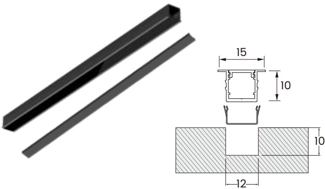
TL4002 recessed mounted
