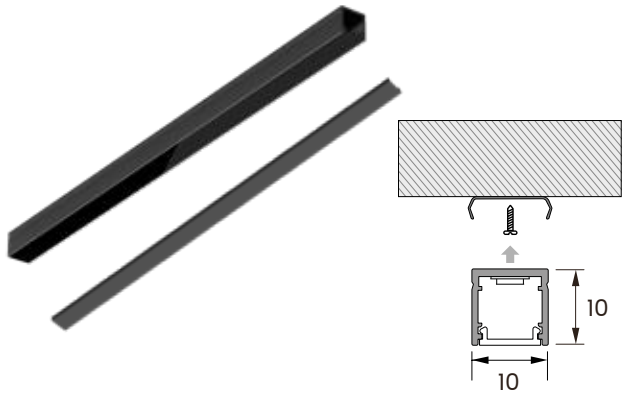
TL4003 surface mounted
